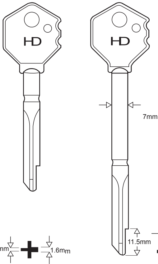
XY4 XKB023
